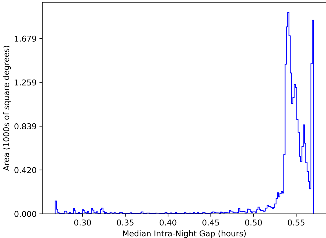
too_elab_heavy_r32_d2_gz_v3.4_10yrs All sky: Median Intra-Night Gap
