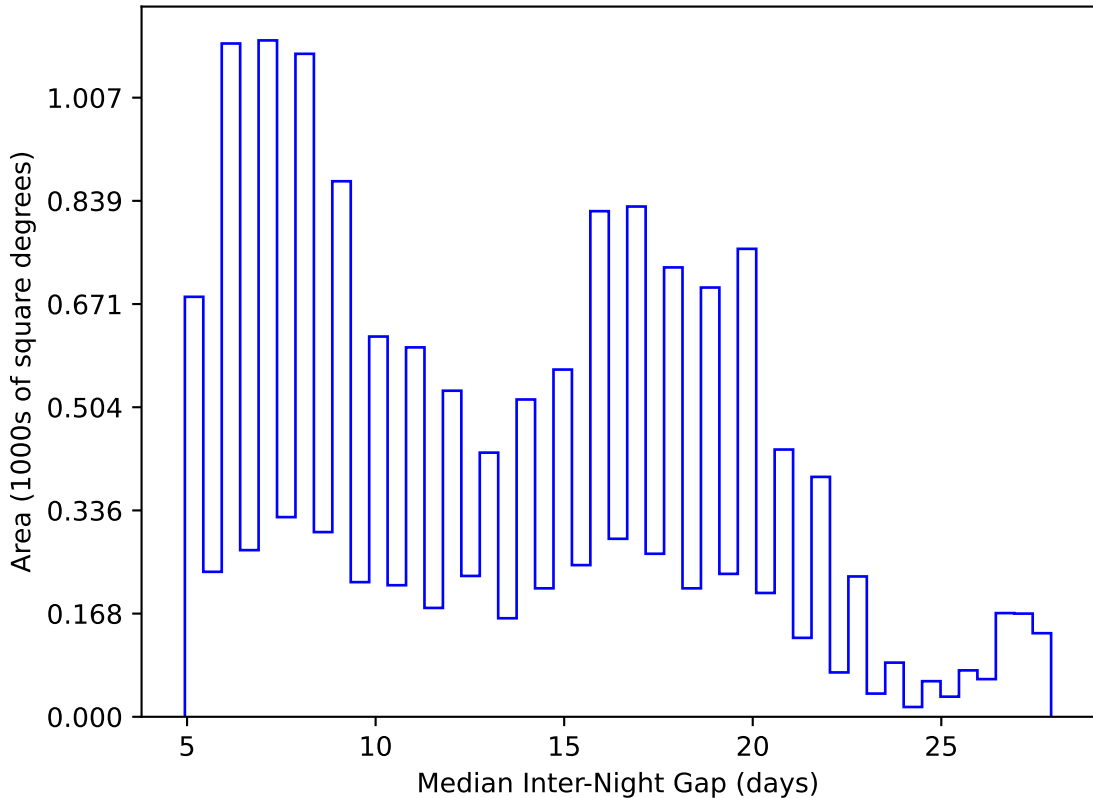
too_elab_heavy_r32_d2_gz_v3.4_10yrs WFD y band: Median Inter-Night Gap
