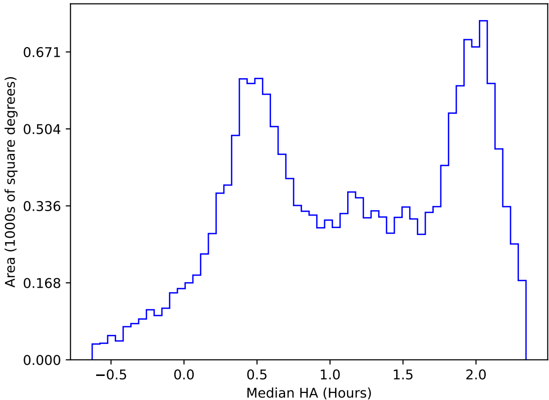
too_elab_heavy_r32_d2_gz_v3.4_10yrs WFD z band: Median HA
