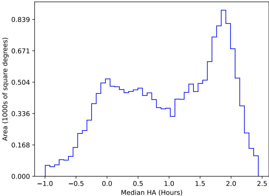
too_elab_heavy_r32_d2_gz_v3.4_10yrs WFD u band: Median HA
