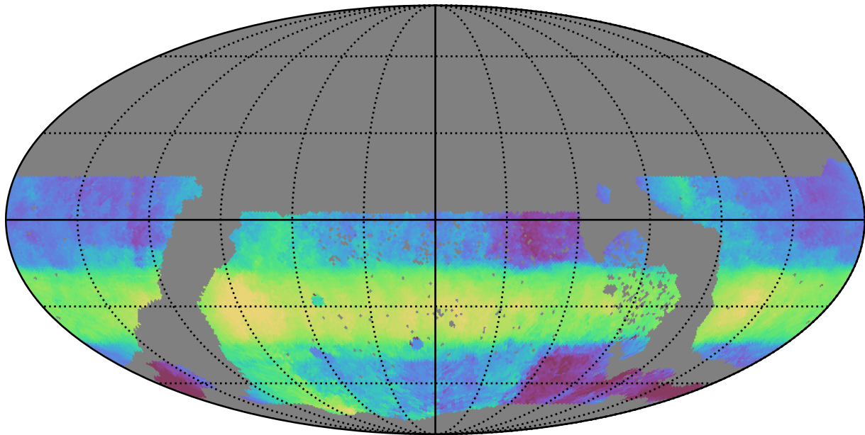
too_elab_heavy_r32_d2_gz_v3.4_10yrs WFD r band: Median HA
