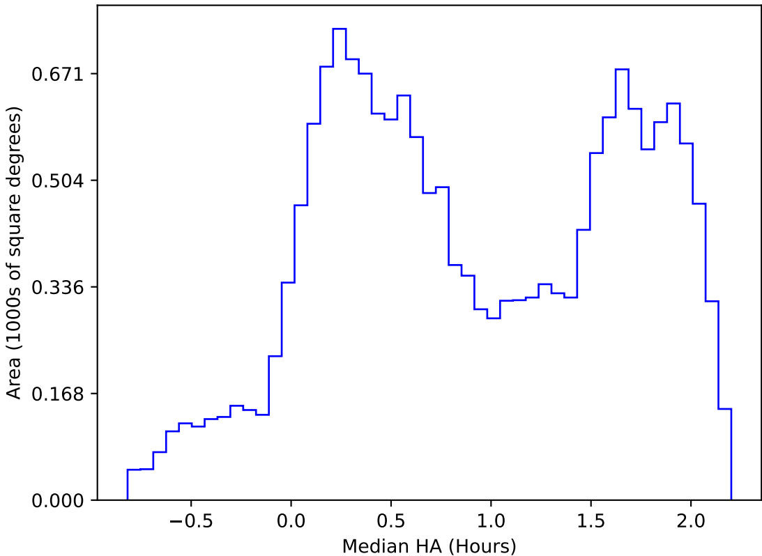
too_elab_heavy_r32_d2_gz_v3.4_10yrs WFD r band: Median HA
