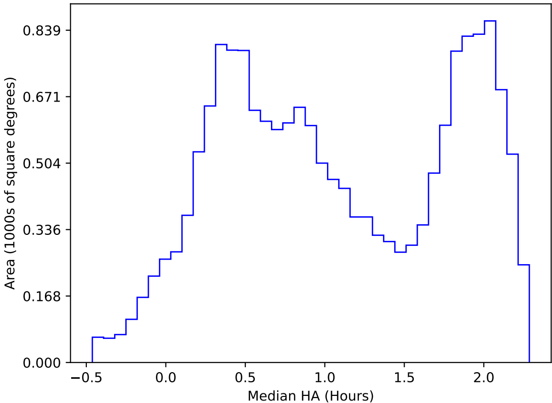
too_elab_heavy_r32_d2_gz_v3.4_10yrs WFD i band: Median HA
