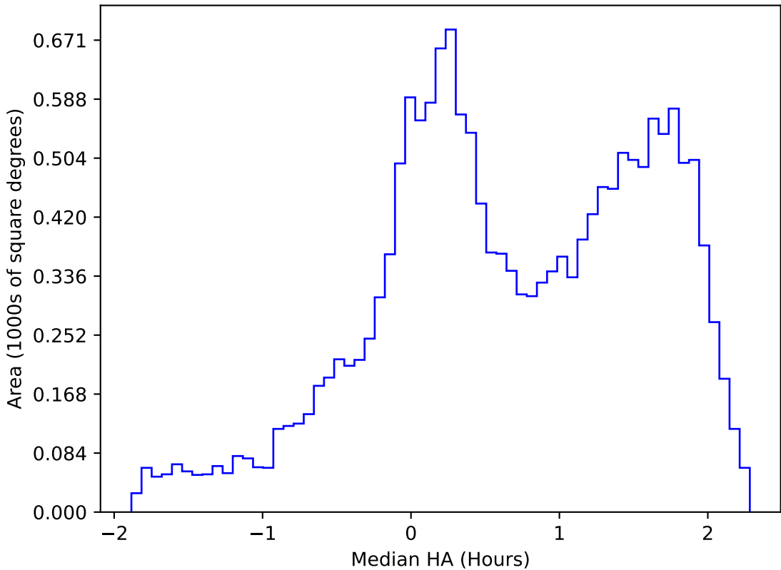
too_elab_heavy_r32_d2_gz_v3.4_10yrs WFD g band: Median HA
