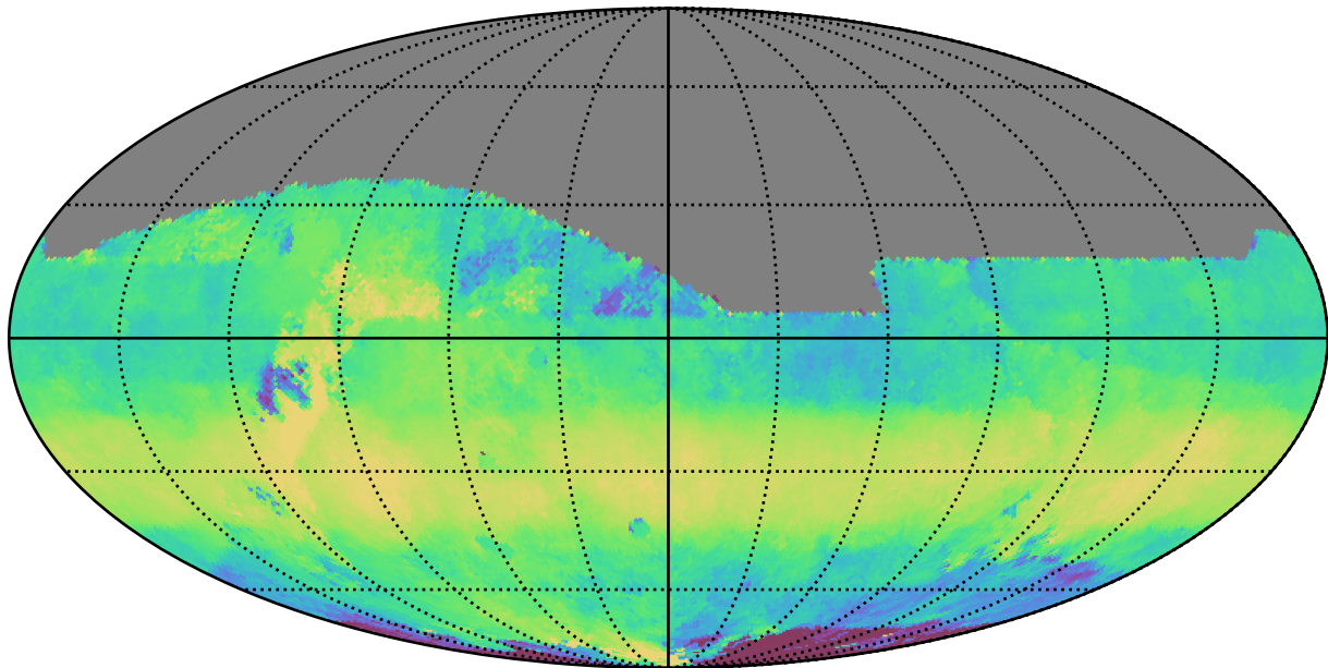
too_elab_heavy_r32_d2_gz_v3.4_10yrs All sky z band: Median HA
