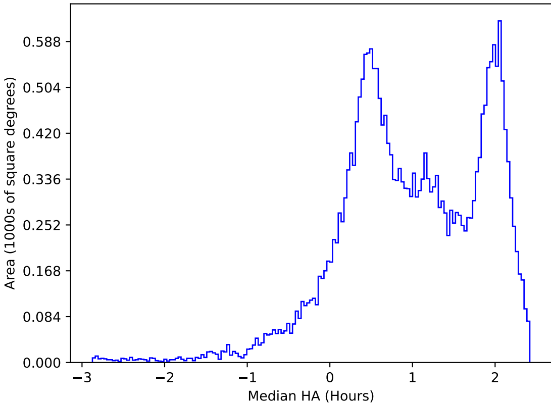
too_elab_heavy_r32_d2_gz_v3.4_10yrs All sky z band: Median HA
