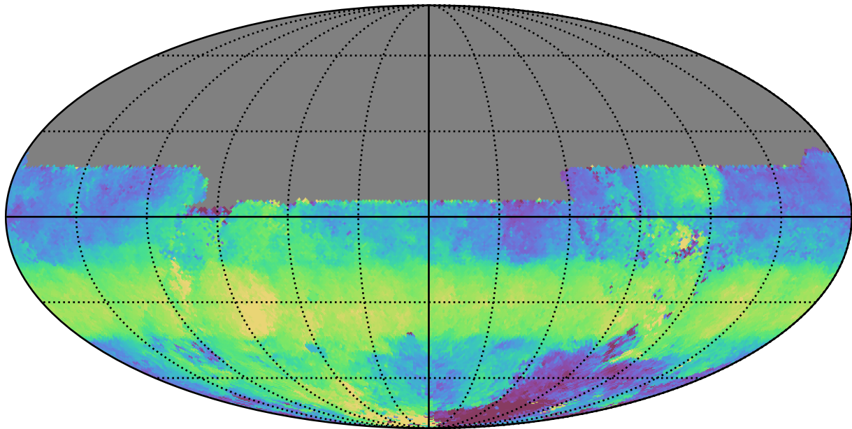
too_elab_heavy_r32_d2_gz_v3.4_10yrs All sky u band: Median HA
