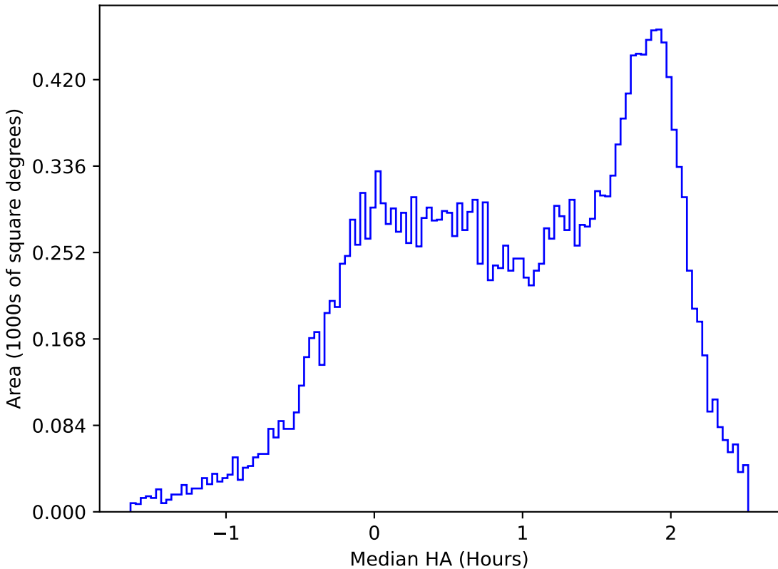
too_elab_heavy_r32_d2_gz_v3.4_10yrs All sky u band: Median HA
