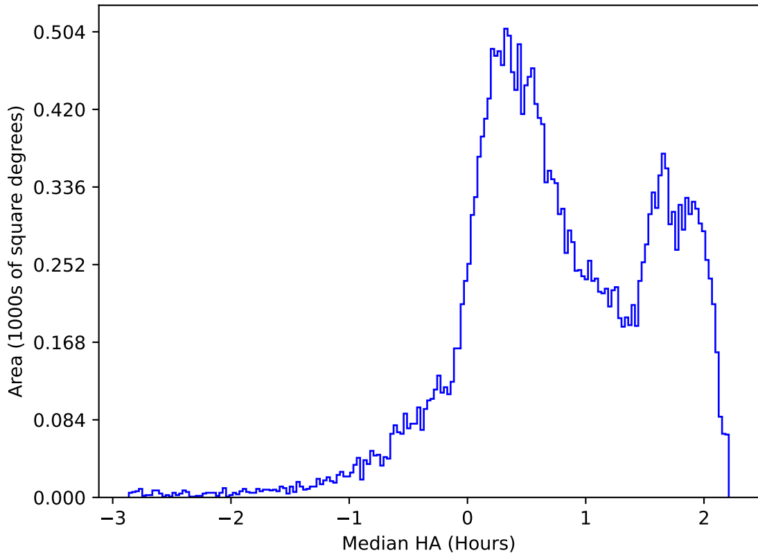
too_elab_heavy_r32_d2_gz_v3.4_10yrs All sky r band: Median HA
