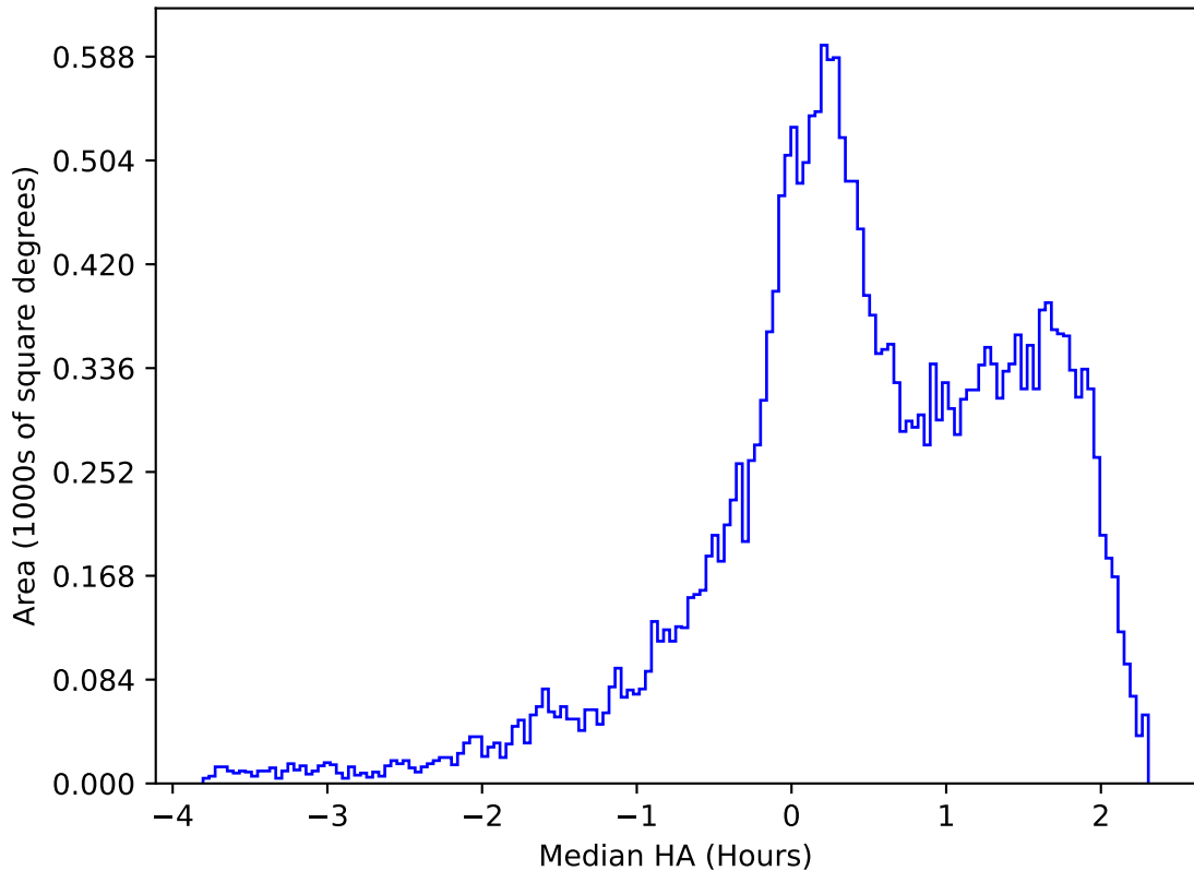
too_elab_heavy_r32_d2_gz_v3.4_10yrs All sky g band: Median HA
