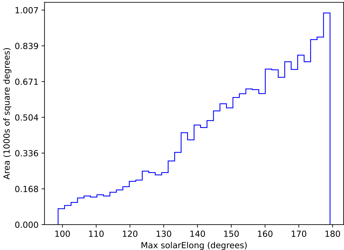
too_elab_heavy_r32_d2_gz_v3.4_10yrs WFD y band: Max solarElong
