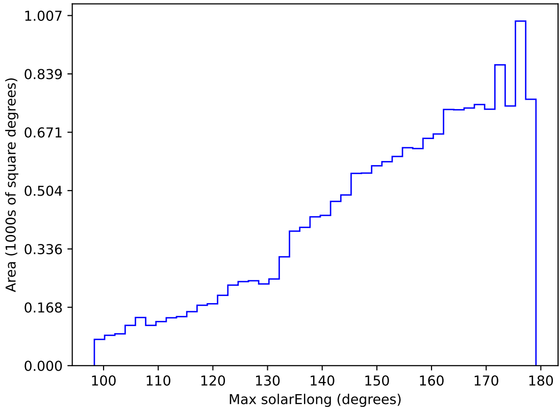
too_elab_heavy_r32_d2_gz_v3.4_10yrs WFD g band: Max solarElong
