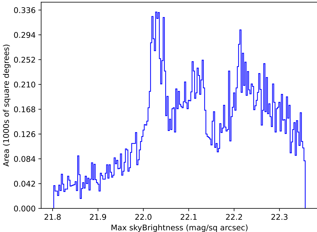
too_elab_heavy_r32_d2_gz_v3.4_10yrs All sky g band: Max skyBrightness
