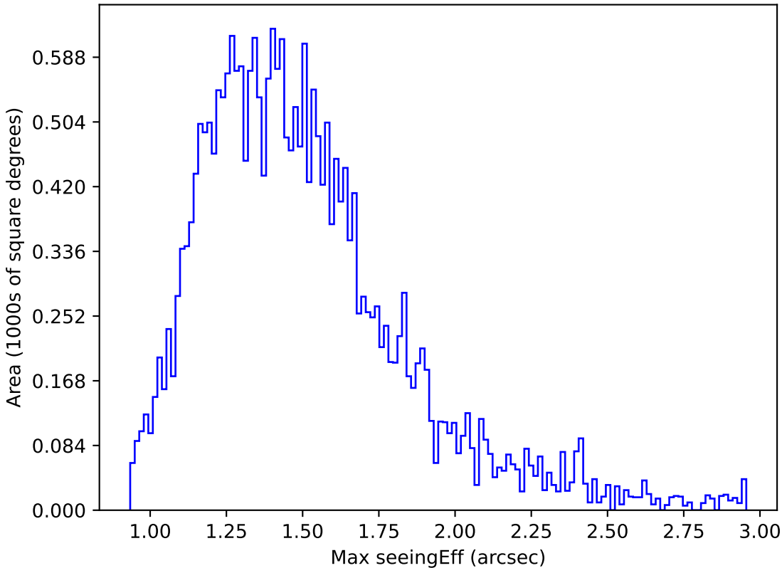
too_elab_heavy_r32_d2_gz_v3.4_10yrs Yr 1 z band: Max seeingEff
