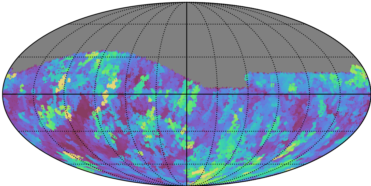
too_elab_heavy_r32_d2_gz_v3.4_10yrs Yr 1 r band: Max seeingEff
