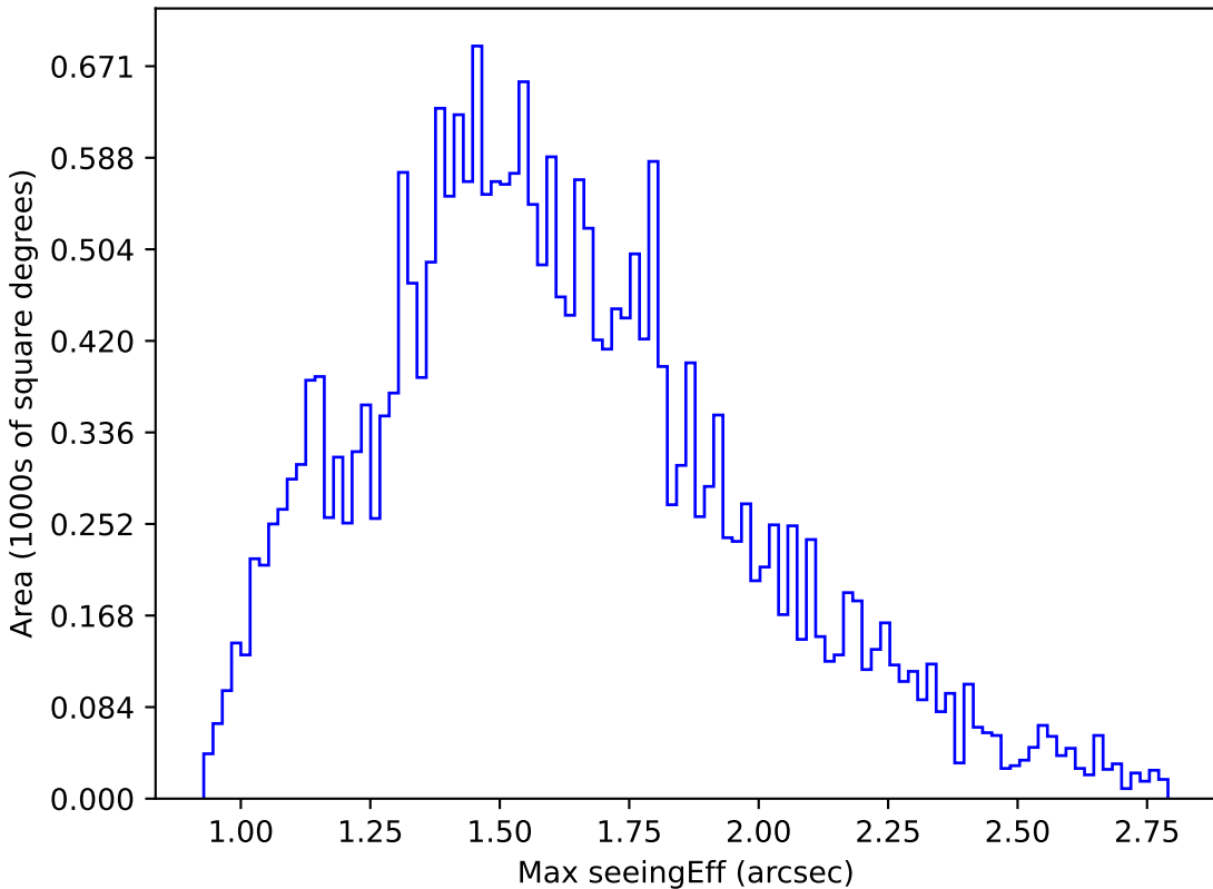
too_elab_heavy_r32_d2_gz_v3.4_10yrs Yr 1 r band: Max seeingEff
