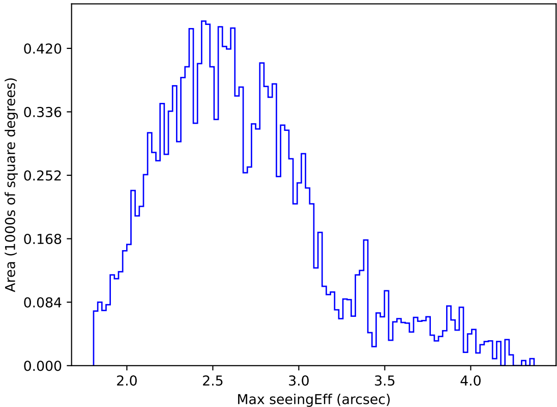
too_elab_heavy_r32_d2_gz_v3.4_10yrs WFD r band: Max seeingEff
