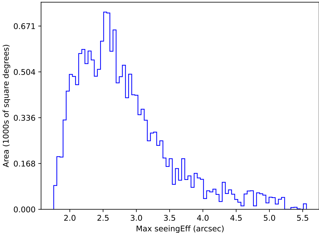
too_elab_heavy_r32_d2_gz_v3.4_10yrs WFD i band: Max seeingEff
