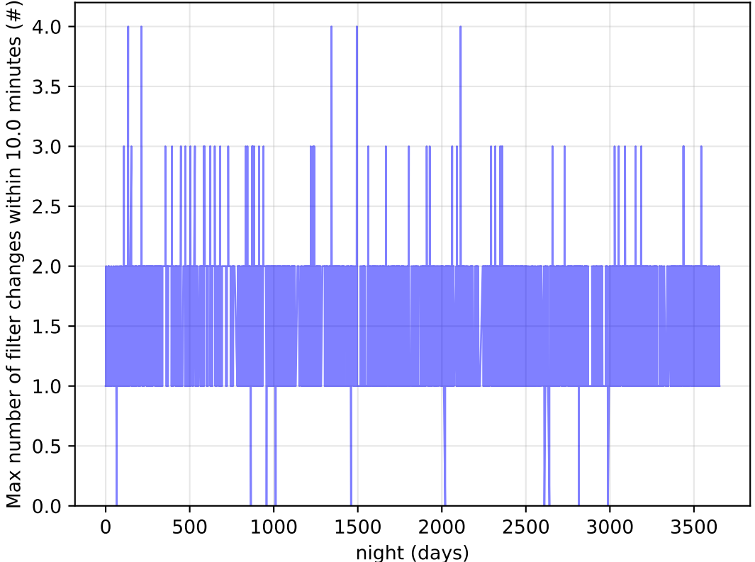
too_elab_heavy_r32_d2_gz_v3.4_10yrs Per Night: Max number of filter changes within 10.0 minutes
