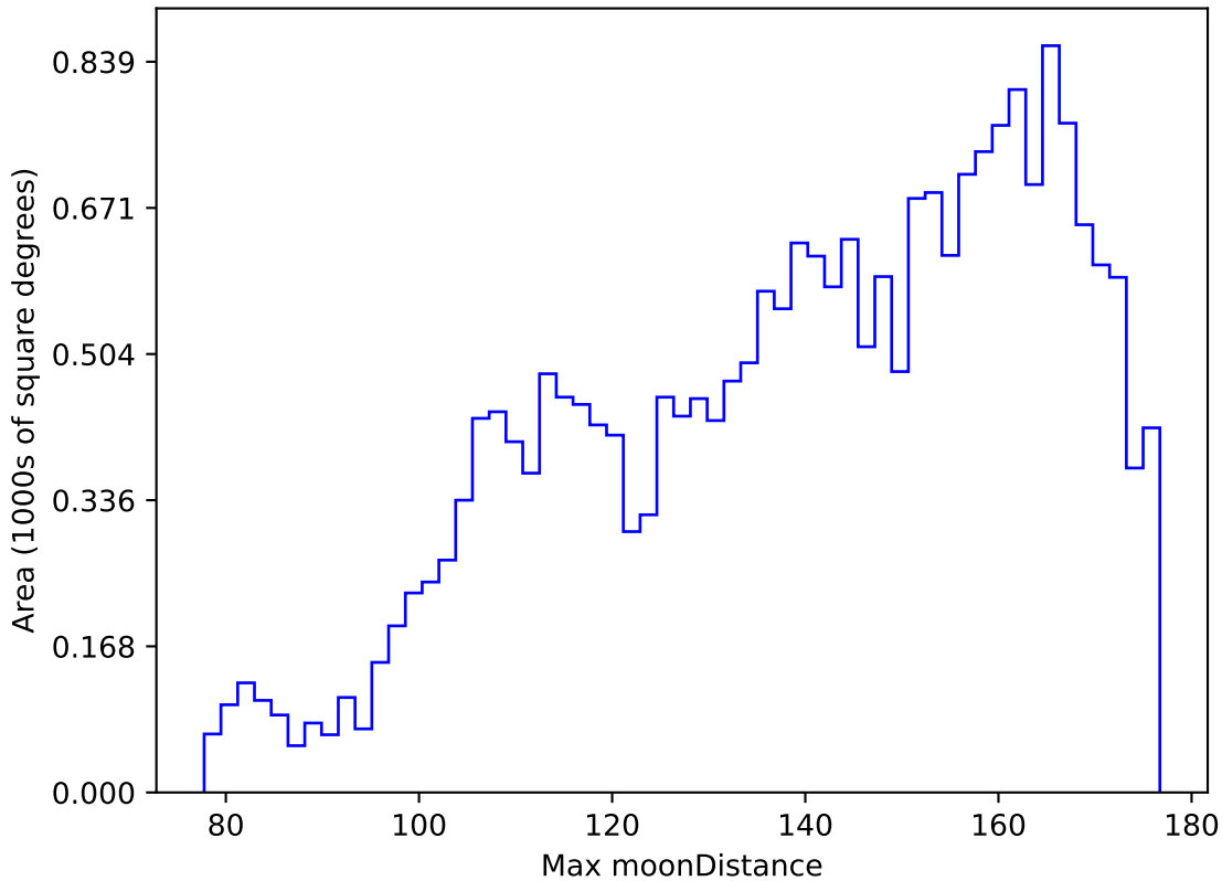
too_elab_heavy_r32_d2_gz_v3.4_10yrs All sky y band: Max moonDistance
