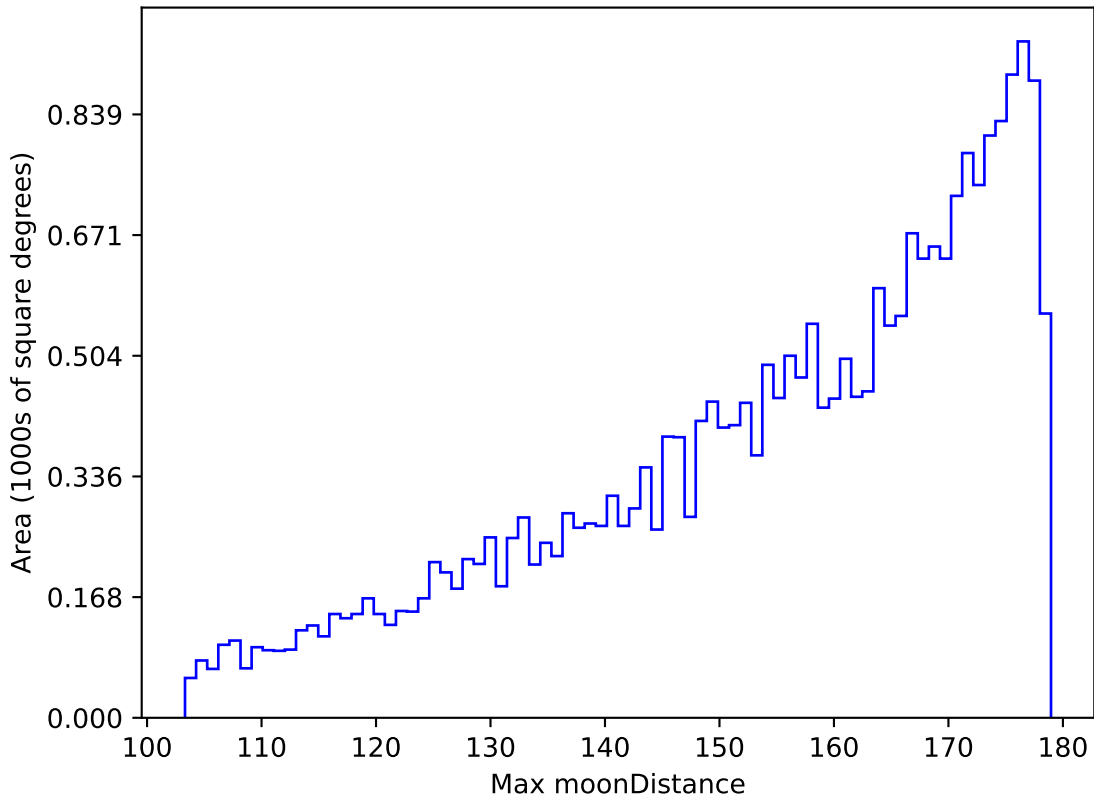
too_elab_heavy_r32_d2_gz_v3.4_10yrs All sky g band: Max moonDistance
