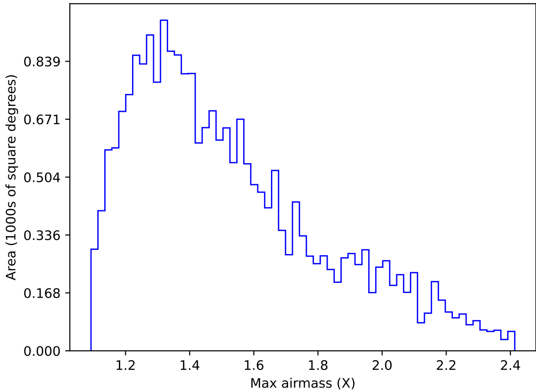
too_elab_heavy_r32_d2_gz_v3.4_10yrs Yr 1 u band: Max airmass
