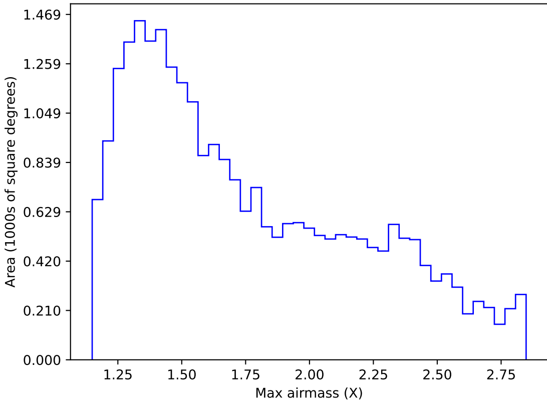
too_elab_heavy_r32_d2_gz_v3.4_10yrs Yr 1 i band: Max airmass
