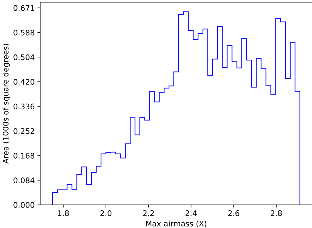
too_elab_heavy_r32_d2_gz_v3.4_10yrs WFD z band: Max airmass
