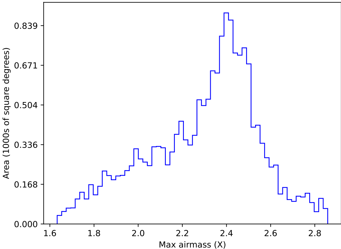
too_elab_heavy_r32_d2_gz_v3.4_10yrs WFD r band: Max airmass
