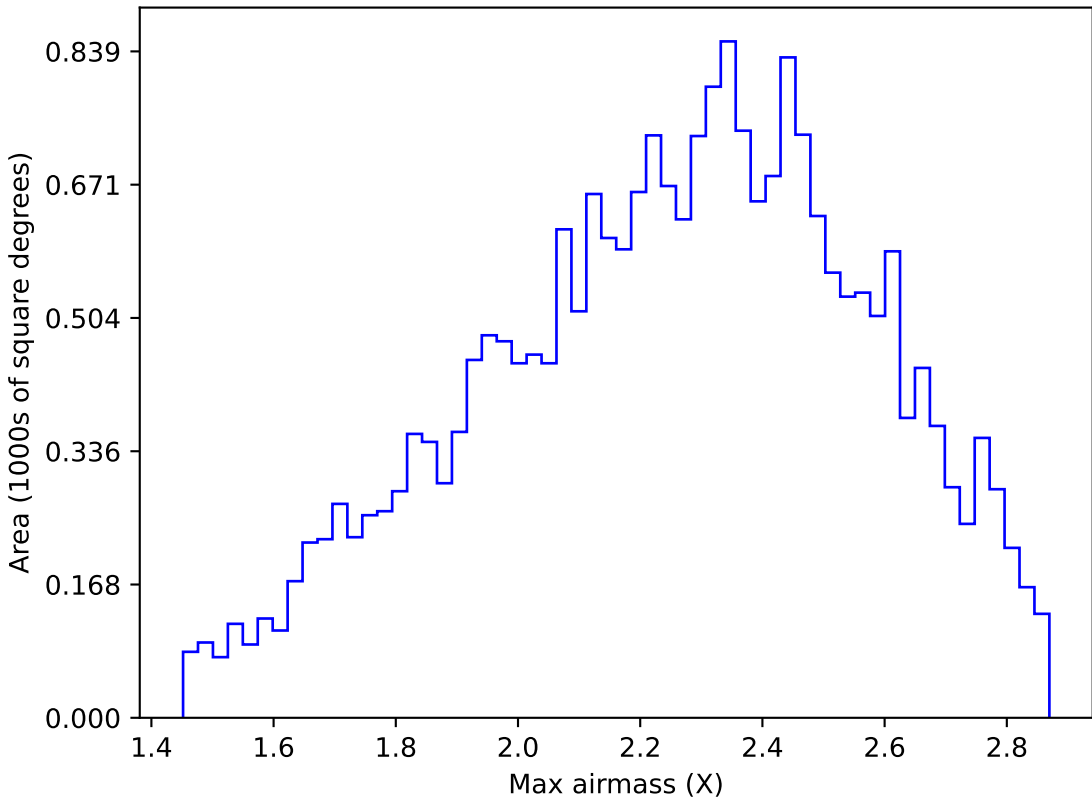
too_elab_heavy_r32_d2_gz_v3.4_10yrs All sky y band: Max airmass
