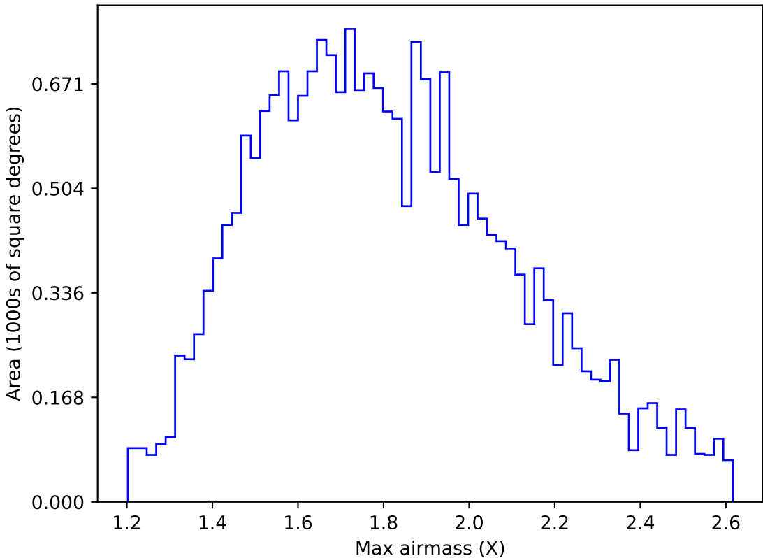
too_elab_heavy_r32_d2_gz_v3.4_10yrs All sky u band: Max airmass
