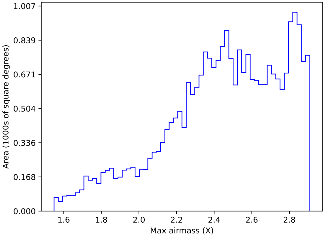
too_elab_heavy_r32_d2_gz_v3.4_10yrs All sky i band: Max airmass
