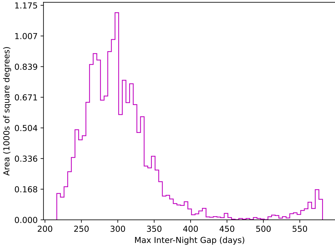
too_elab_heavy_r32_d2_gz_v3.4_10yrs WFD z band: Max Inter-Night Gap
