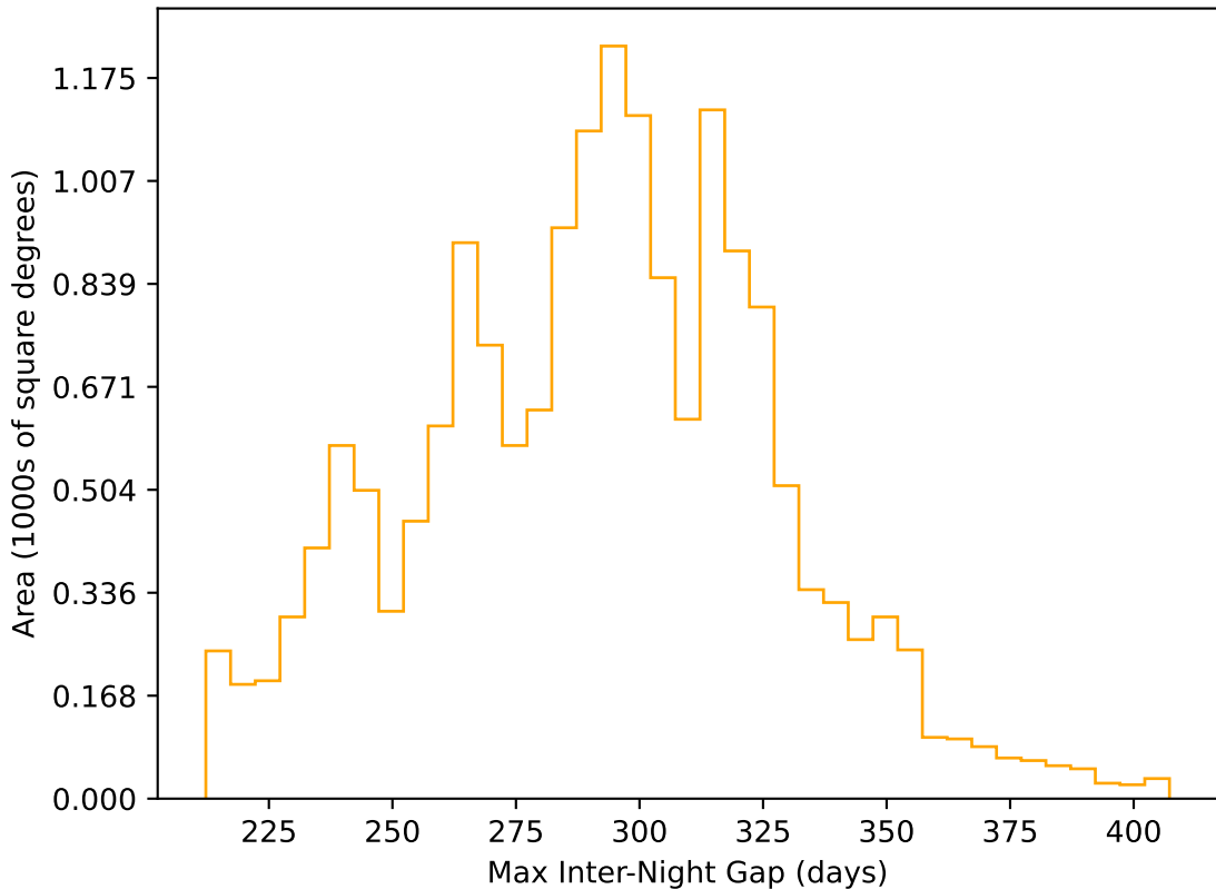
too_elab_heavy_r32_d2_gz_v3.4_10yrs WFD r band: Max Inter-Night Gap
