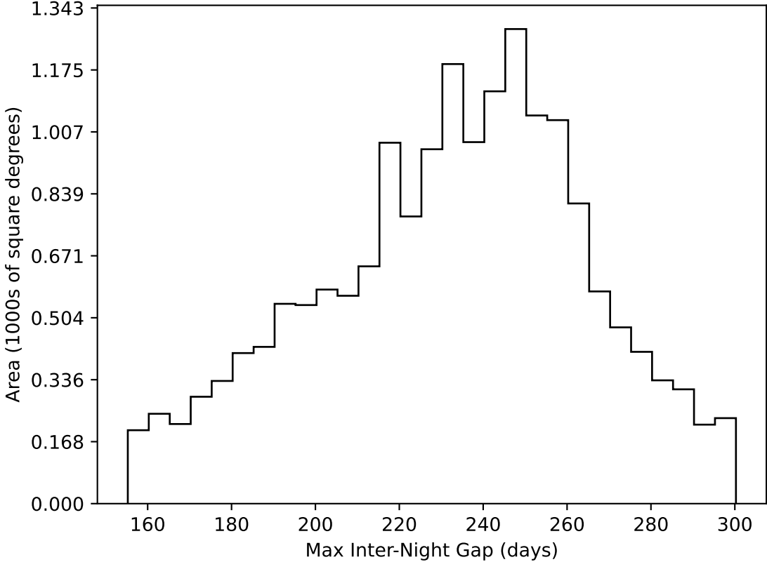
too_elab_heavy_r32_d2_gz_v3.4_10yrs WFD all bands: Max Inter-Night Gap
