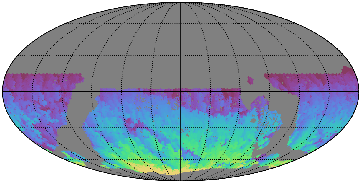
too_elab_heavy_r32_d2_gz_v3.4_10yrs WFD z band: Max HA
