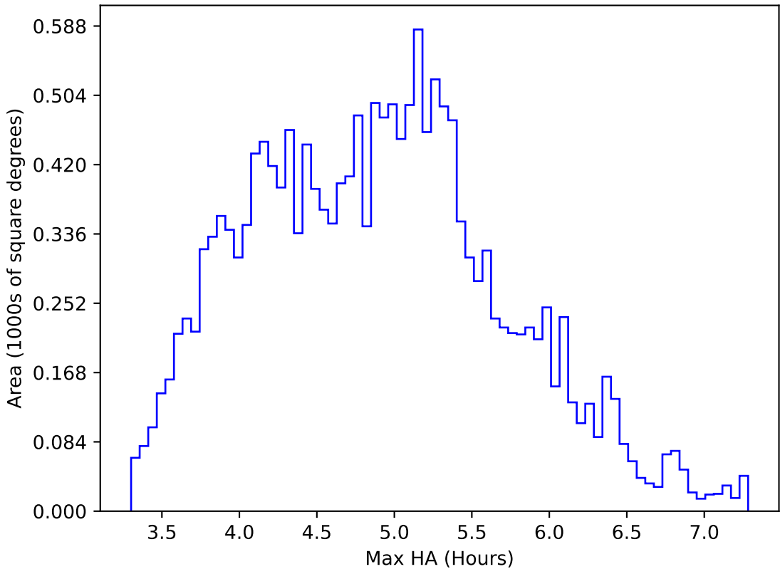
too_elab_heavy_r32_d2_gz_v3.4_10yrs WFD z band: Max HA
