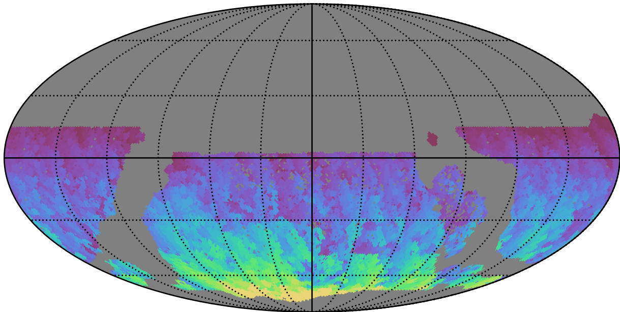
too_elab_heavy_r32_d2_gz_v3.4_10yrs WFD y band: Max HA
