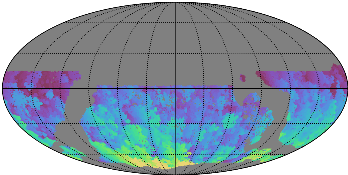
too_elab_heavy_r32_d2_gz_v3.4_10yrs WFD g band: Max HA
