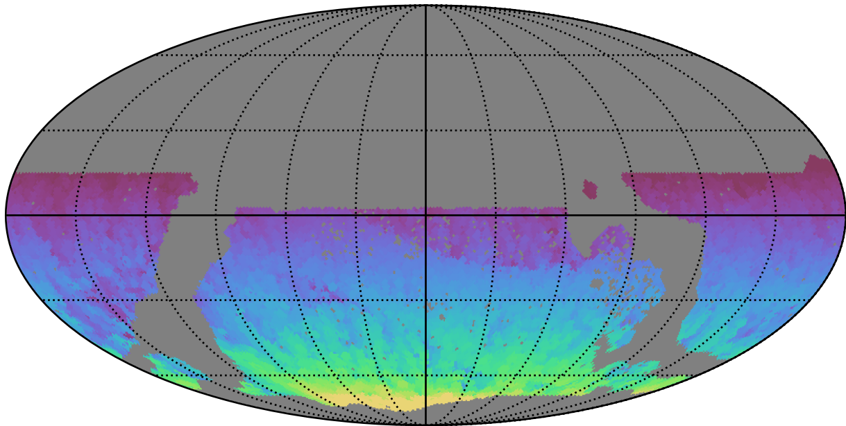
too_elab_heavy_r32_d2_gz_v3.4_10yrs WFD all bands: Max HA
