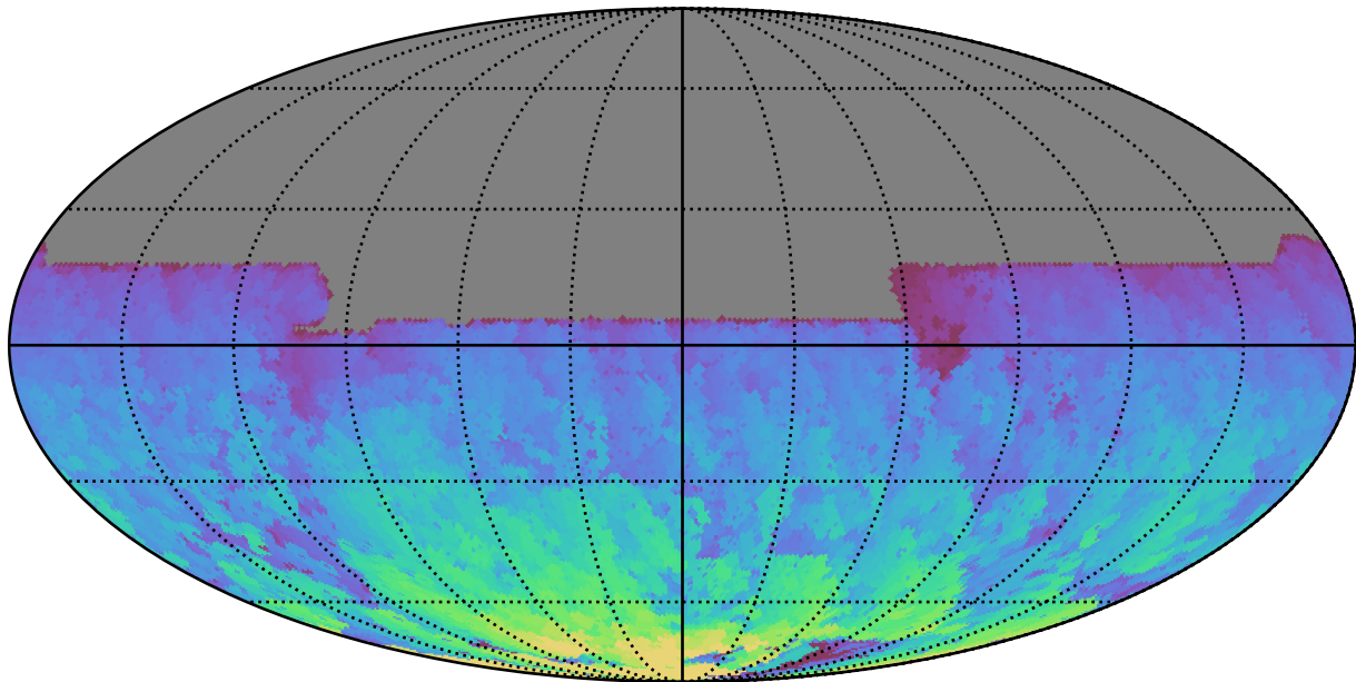
too_elab_heavy_r32_d2_gz_v3.4_10yrs All sky y band: Max HA
