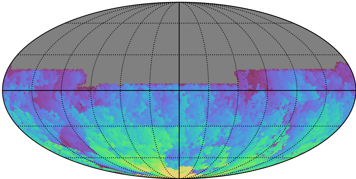
too_elab_heavy_r32_d2_gz_v3.4_10yrs All sky u band: Max HA
