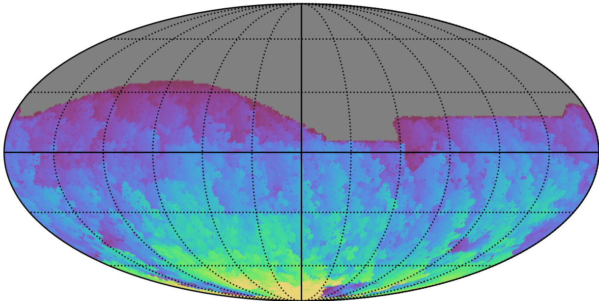
too_elab_heavy_r32_d2_gz_v3.4_10yrs All sky r band: Max HA
