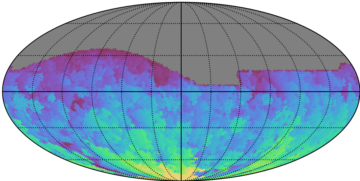
too_elab_heavy_r32_d2_gz_v3.4_10yrs All sky g band: Max HA
