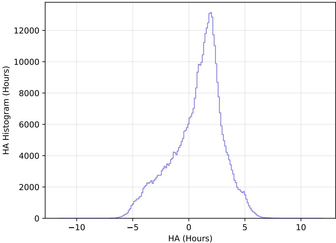
too_elab_heavy_r32_d2_gz_v3.4_10yrs WFD z band: HA Histogram
