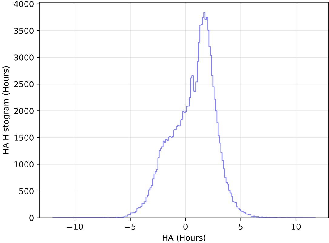
too_elab_heavy_r32_d2_gz_v3.4_10yrs WFD u band: HA Histogram
