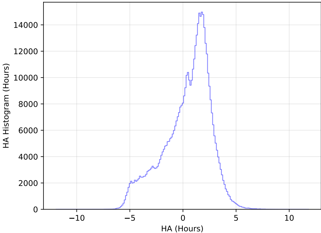
too_elab_heavy_r32_d2_gz_v3.4_10yrs WFD r band: HA Histogram
