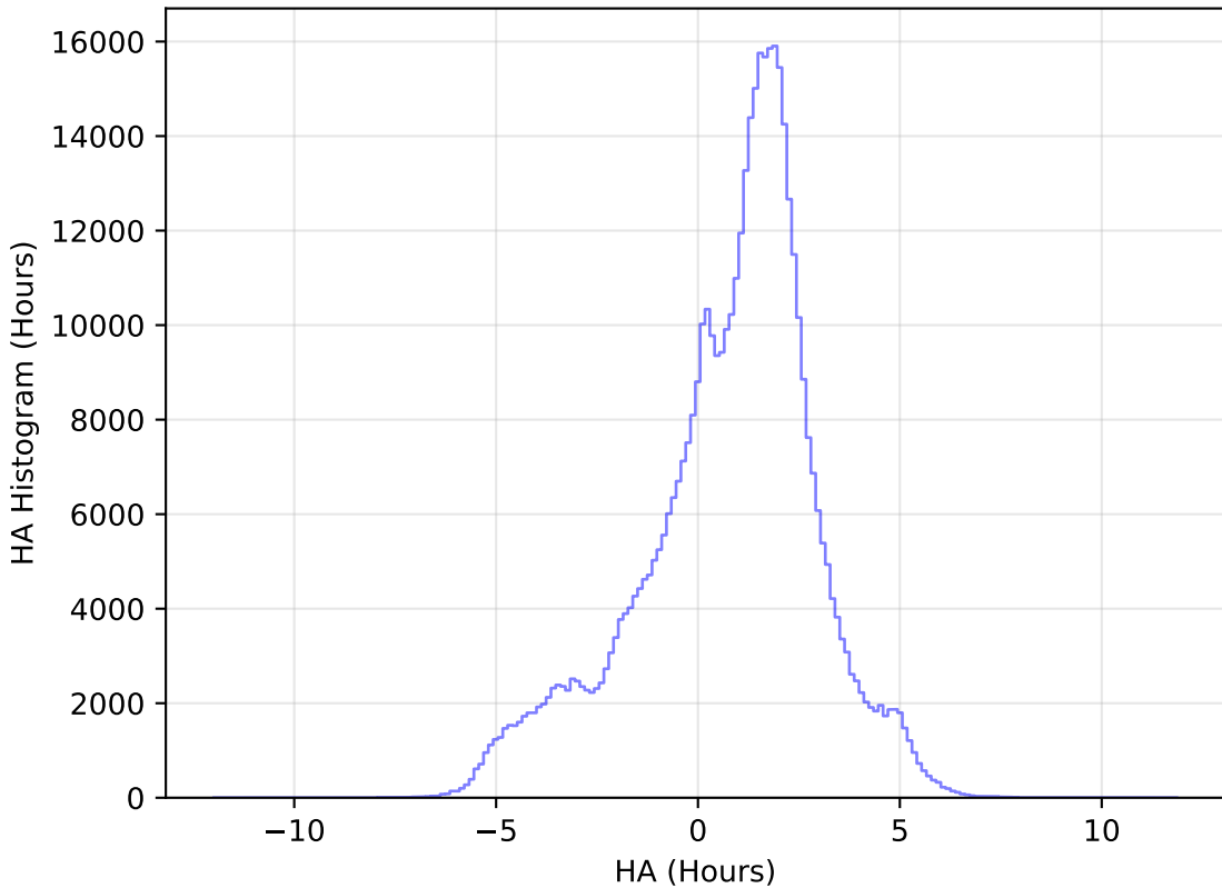
too_elab_heavy_r32_d2_gz_v3.4_10yrs WFD i band: HA Histogram
