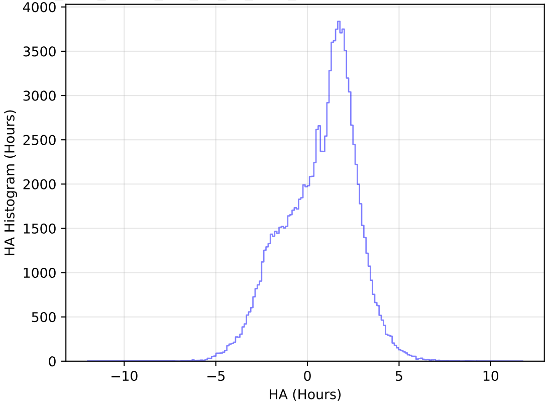
too_elab_heavy_r32_d2_gz_v3.4_10yrs All sky u band: HA Histogram
