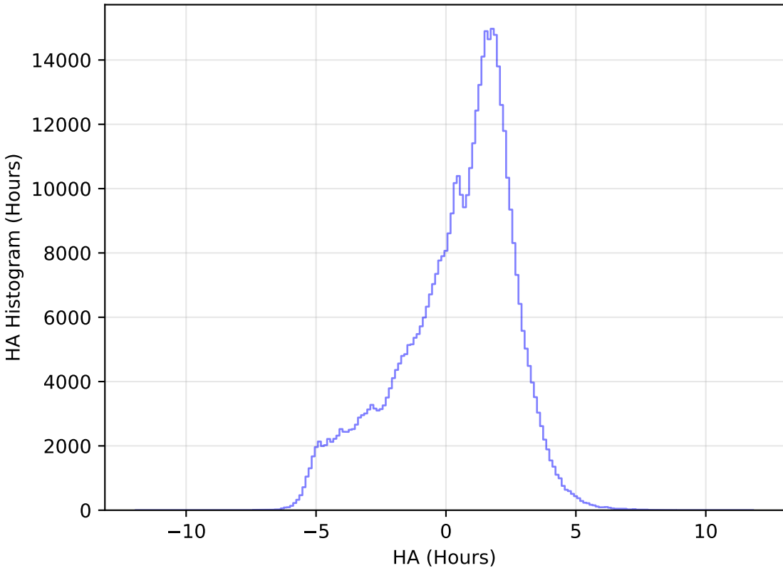
too_elab_heavy_r32_d2_gz_v3.4_10yrs All sky r band: HA Histogram
